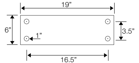
Bollard base detail
